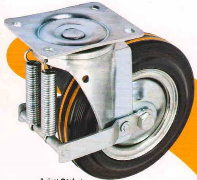
Swivel Castors with Spring Lock RG/PT/CT/200/R/TG/SA
