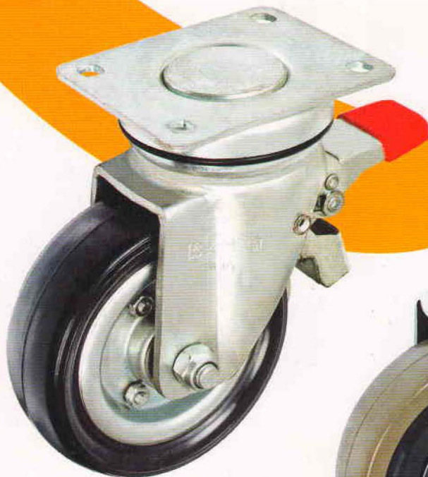
Heavy duty Castor with Taper Roller bearing secondary race RGM5/PT/CT/150/R/BK
