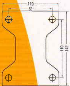
ALTERNATE DIMENSIONS OF 160 FIXED BRACKETS
