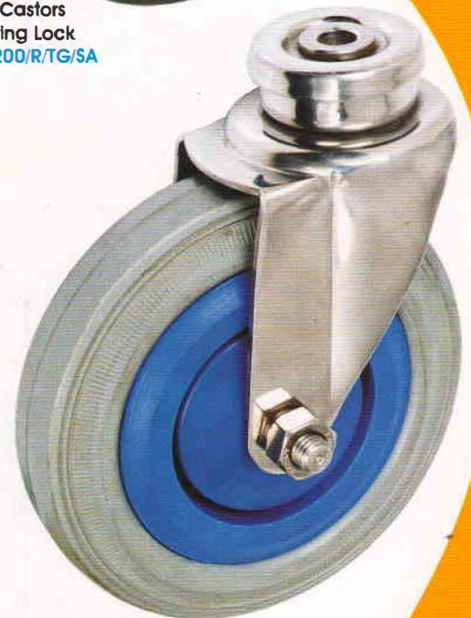
Precision ball bearing Swivel bolt hole 12.5mm RGG/BH/CT/200/BP/TG
