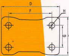
ALTERNATE DIMENSIONS OF 160 FIXED BRACKETS
