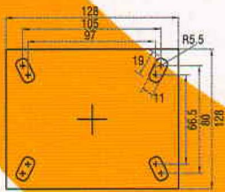
TOP PLATE-BOLT HOLE CENTERS AS PER I.S.I. & OUR STANDARD (COMBINED)
